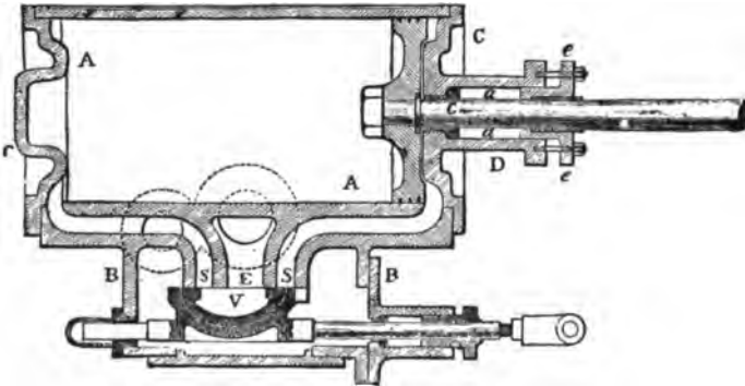
FIG. 237.—Section through a Steam Cylinder and Valve Chest, showing parts. A is the cylinder; B, the steam chest; C and C, the cylinder heads; D, the stuffing box; a and a, the packing gland; c, the piston rod; E, the exhaust port; S and S, the steam ports; V, the slide valve; e, e, the packing gland, held in place by screws in this engine.
